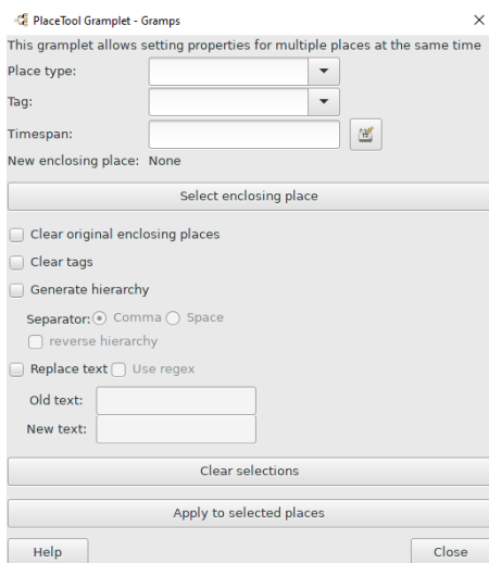
Fig. Isotammi.9 PlaceTool Gramplet - detached
