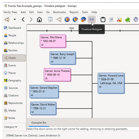
Fig. TimelinePedigreeView.1 Timeline pedigree View - Addon for Charts Category - display example
