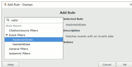
Fig. Isotammi.27 Events with Invalid Date Rule
