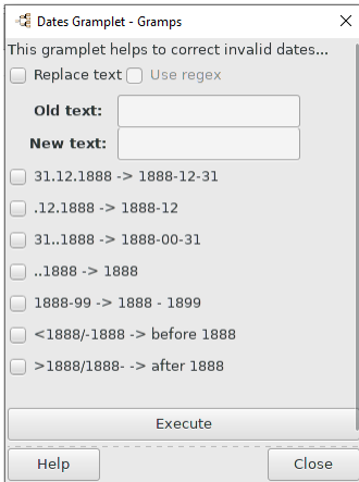
Fig. Isotammi.8 Dates Gramplet - detached
