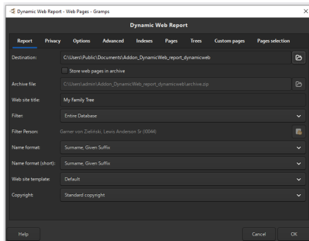
Dynamic Web Report - Web Pages - Report tab defaults
